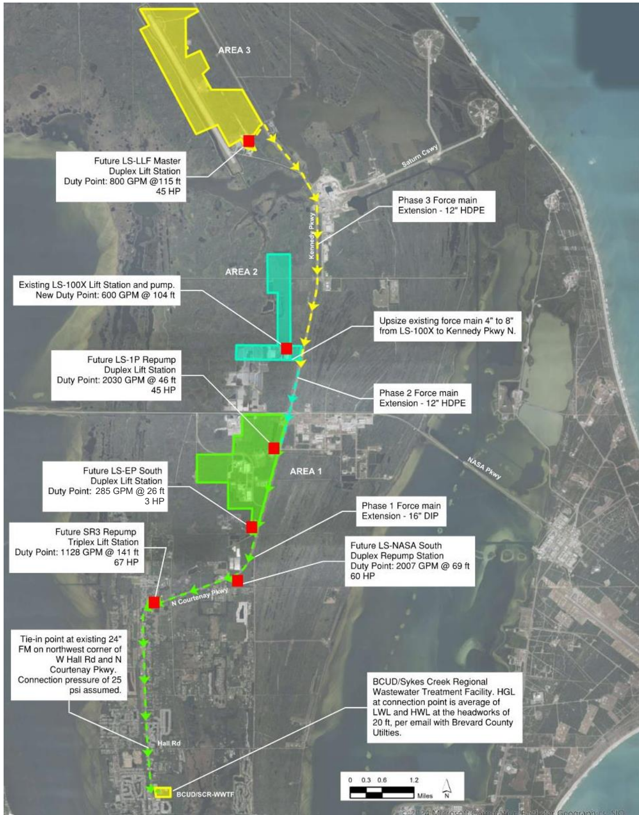
Figure 4-1: Collection System Improvements
