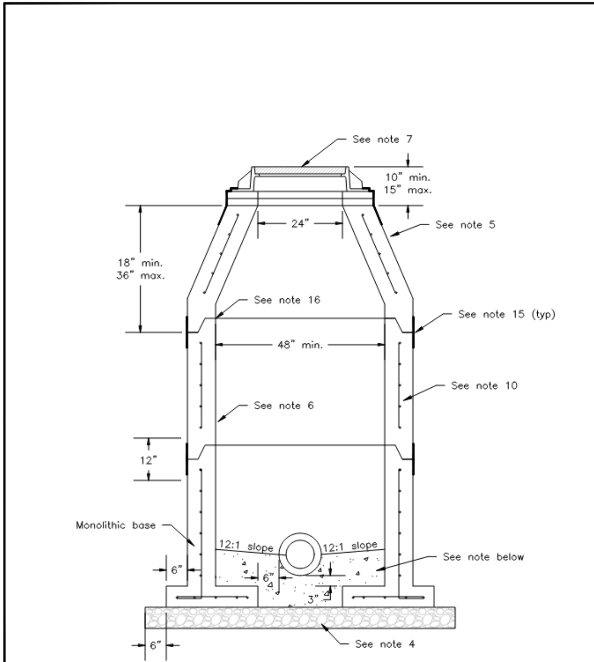
Figure 18 - Dog House Manhole Detail (US-26)
