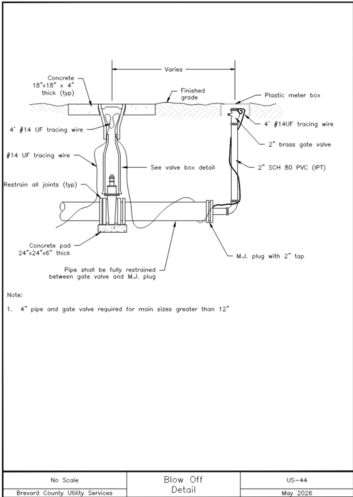
Image Description US-44 Blow Off Detail
