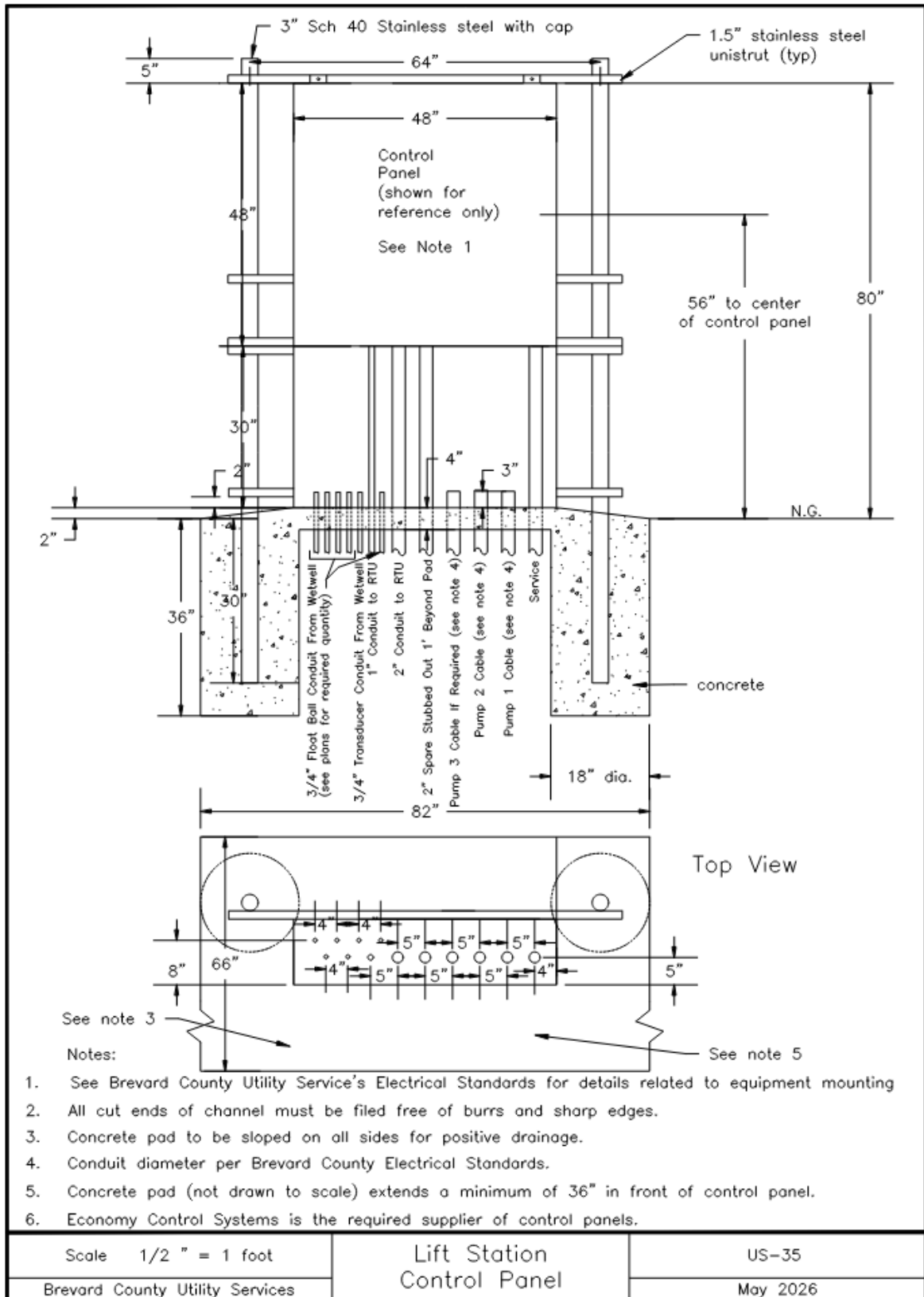
Image Description US-35 Lift Station Control Panel
