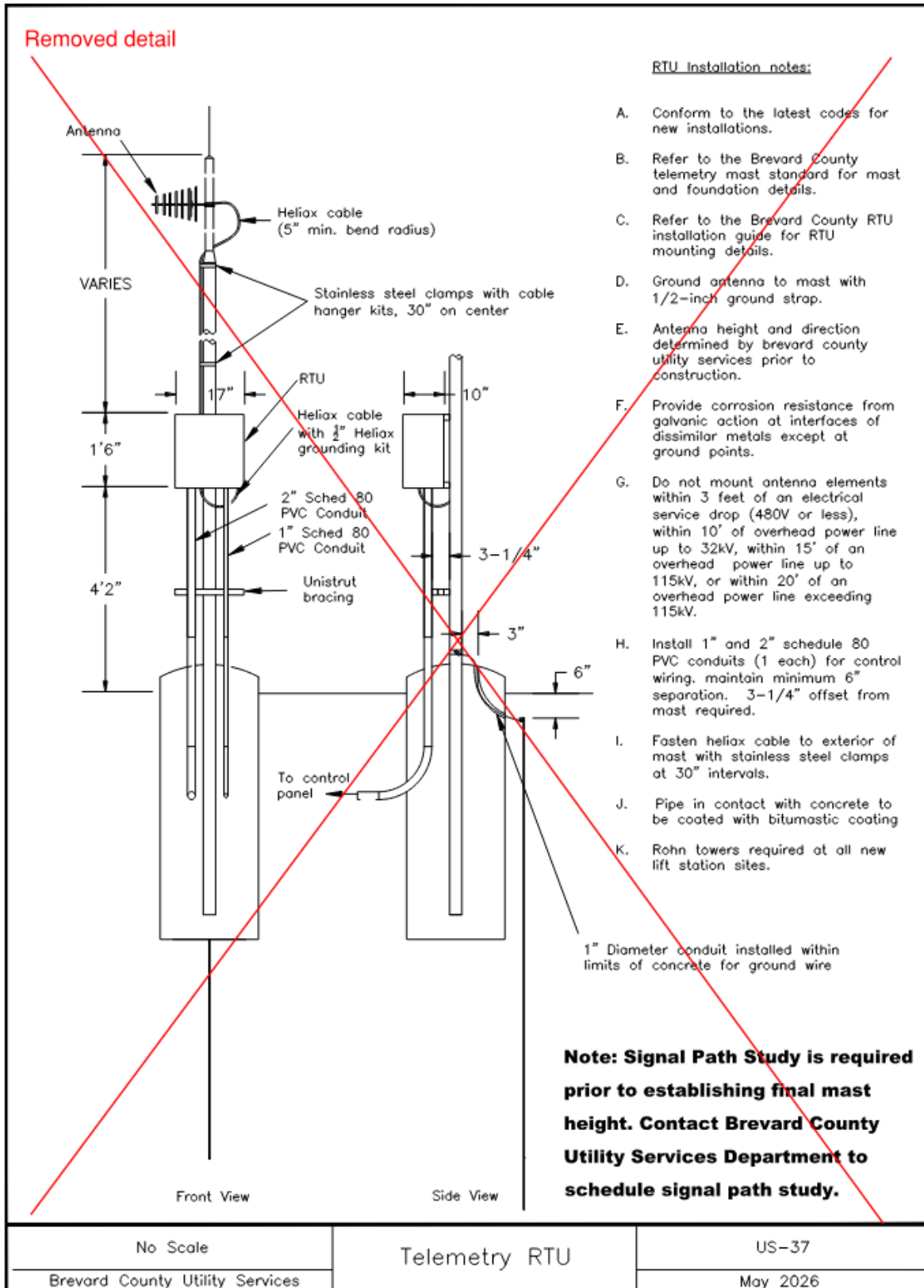
Figure 35 - Telemetry RTU Detail Reserved for Future Use (US-37)
