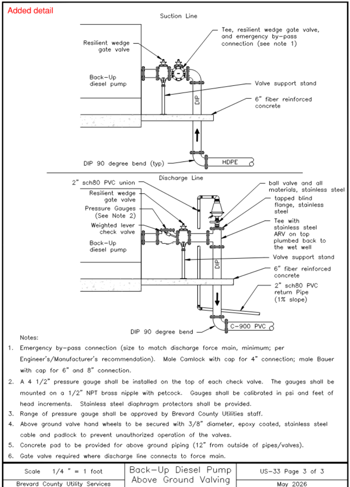
Image Description US-33 Page 3 of 3 Back-Up Diesel Pump Above Ground Valving
