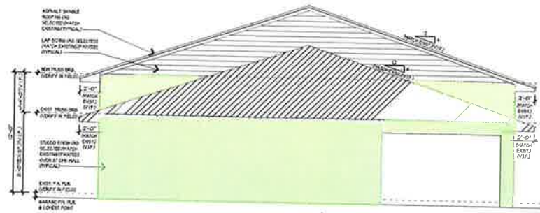
SIDE (NORTH) ELEVATION SCALE: 1/4" = 1'-0"
