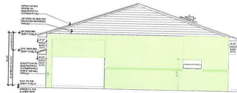
SIDE (SOUTH) ELEVATION SCALE: 1/4" = 1'-0"
